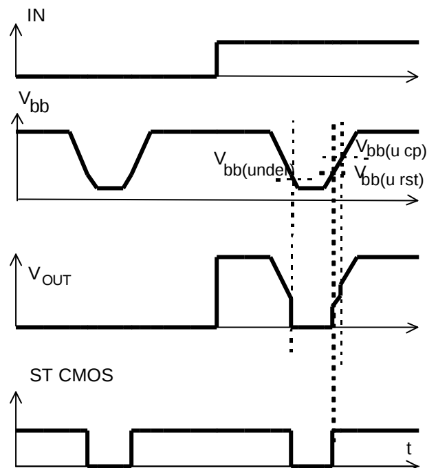
Figure 6a: Undervoltage:
