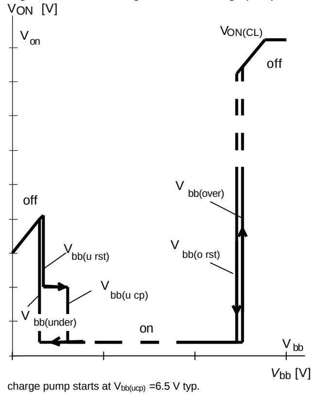
Figure 7a: Overvoltage:
