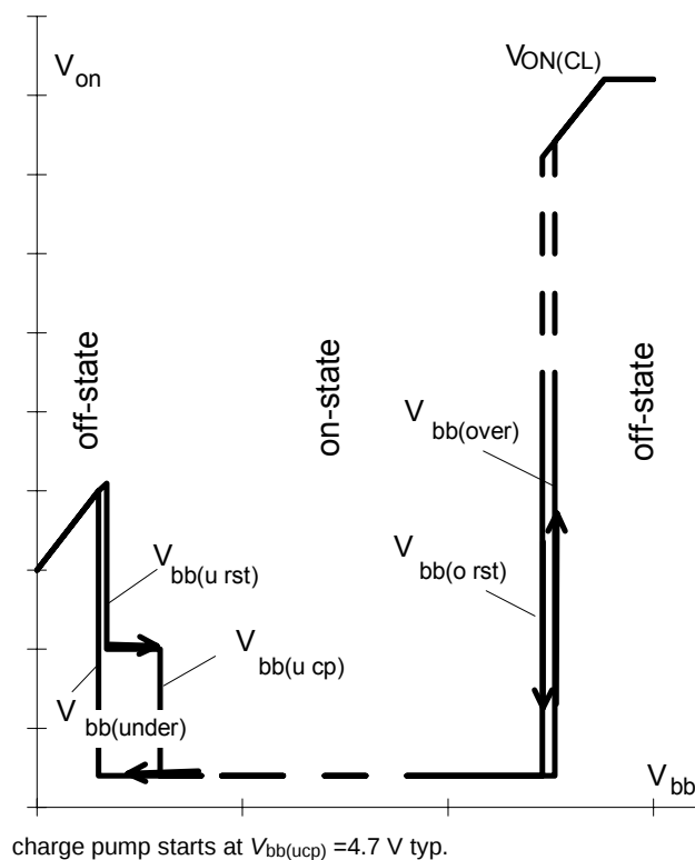
Figure 7a: Overvoltage:
