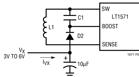
Figure 8. Lower V_{BOOST}
