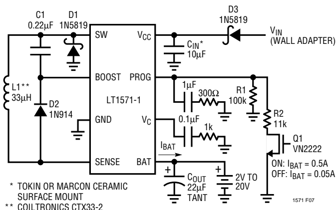
Figure 7. Charging NiMH or NiCd Batteries with Constant Current (Efficiency at 0.5A \approx 90%)
