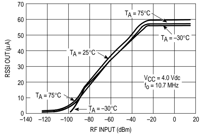
Figure 4. RSSI versus RF Input
