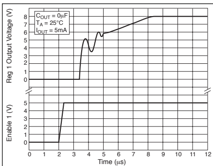
Regulator 1 Startup
