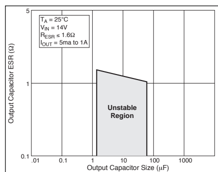
Regulator 1 Stability
