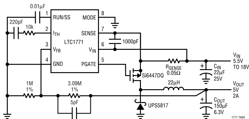
5V/2A Regulator with Burst Mode Operation Disabled
