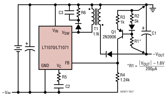
Negative Input/Negative Output Flyback Converter
