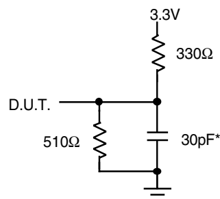
Figure 2. Output Load
