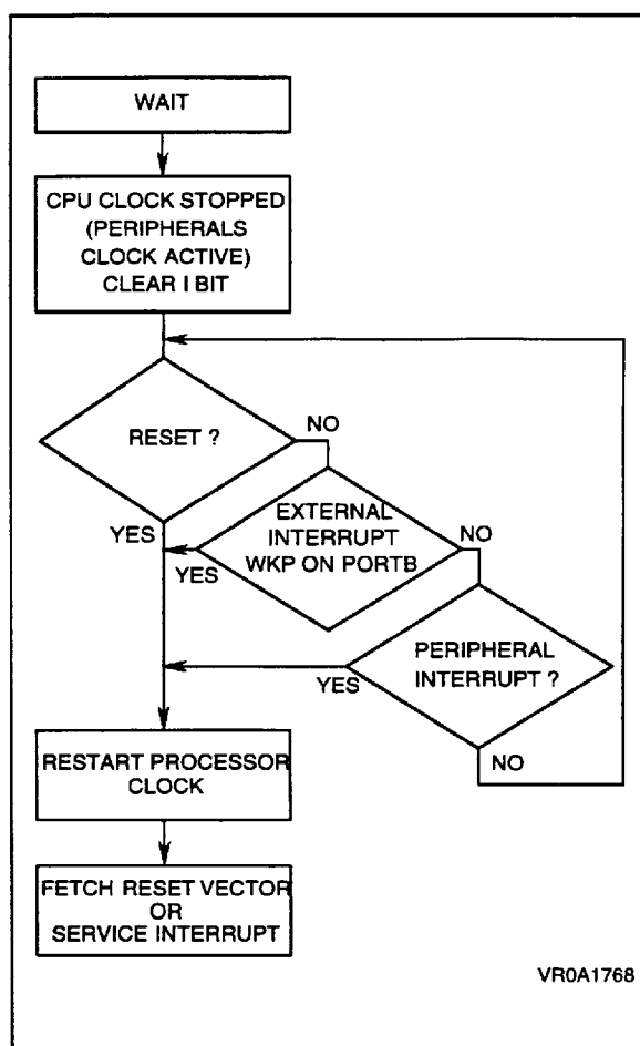
Figure 12b. WAIT Flow Chart
