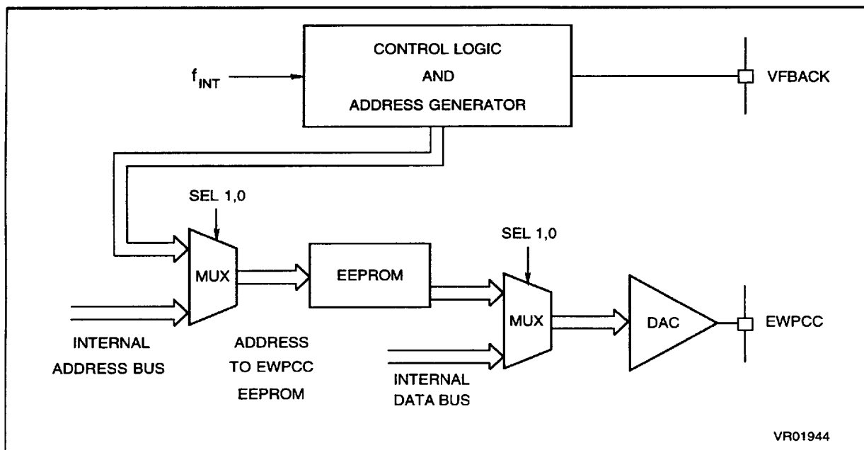
Figure 36. EWPCCE Block Diagram
