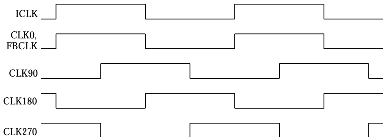
Figure 1. Phase alignment of input and output clocks. (x1 multiplier)
