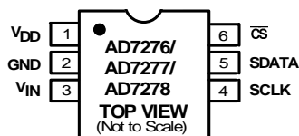
6-Lead TSOT
