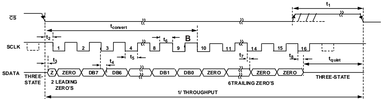
Figure 18. AD7278 Serial Interface Timing Diagram
