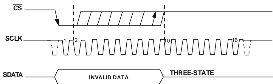
Figure 13. Entering Power Down Mode
