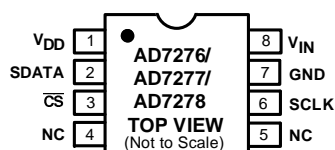
8-Lead MSOP
