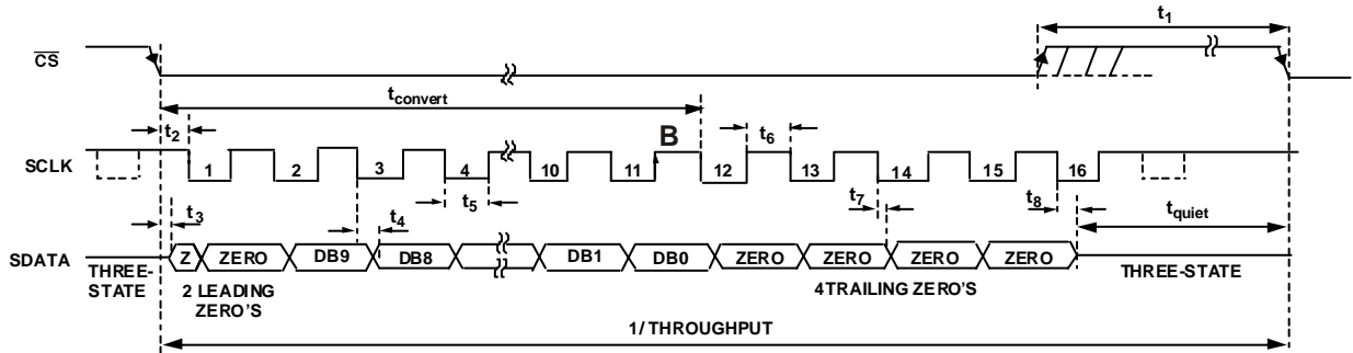
Figure 17. AD7277 Serial Interface Timing Diagram
