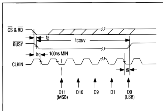
Figure 7. MX7672 \overline{RD} and \overline{CLKIN} for Synchronous Operation and conversion time of 12.5 clock cycles
