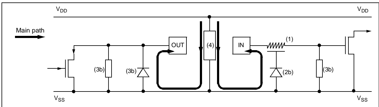
Figure 86. Multisupply Configuration
