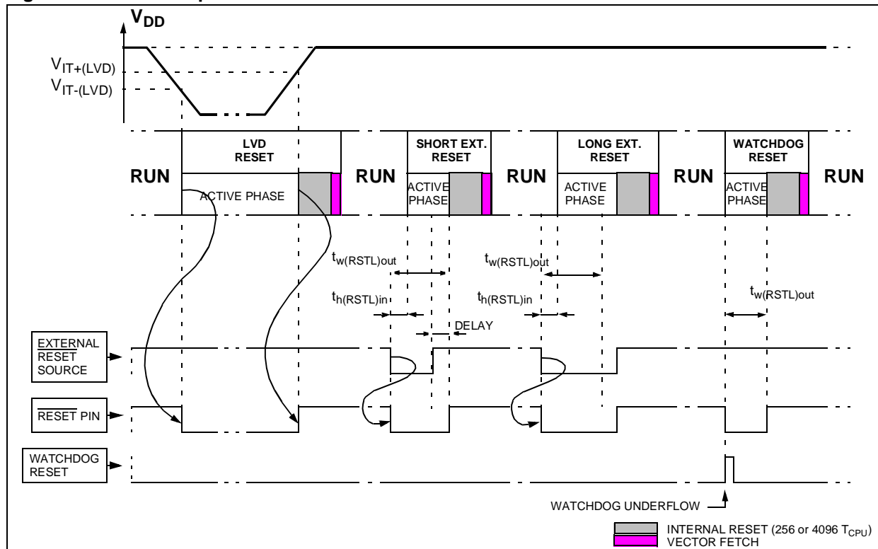
Figure 12. RESET Sequences
