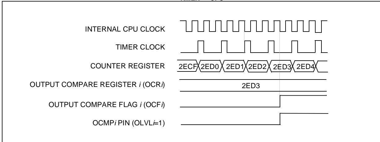
Figure 48. Output Compare Timing Diagram, f_{\text{TIMER}} = f_{\text{CPU}}/4
