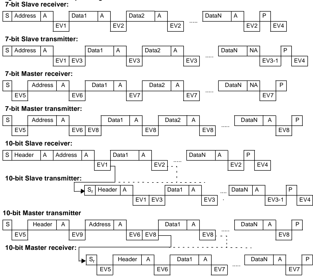
Figure 63. Transfer Sequencing
