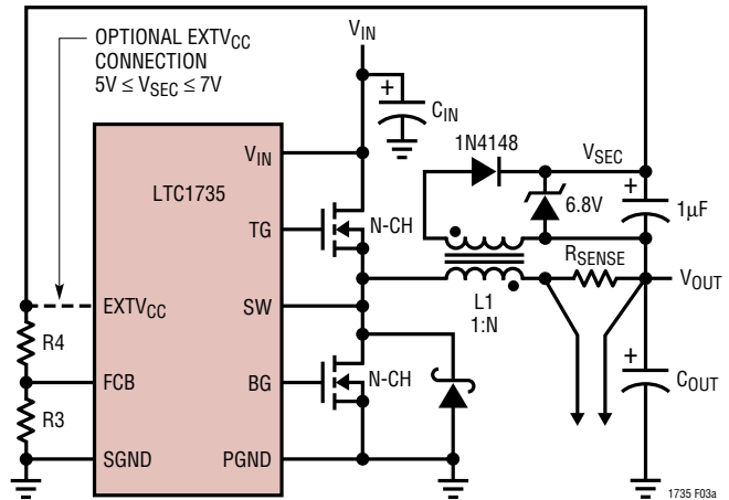
Figure 3a. Secondary Output Loop and EXTV CC Connection
