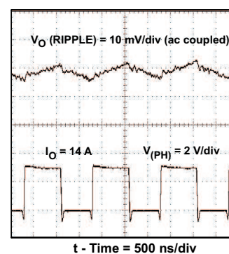
OUTPUT VOLTAGE RIPPLE
