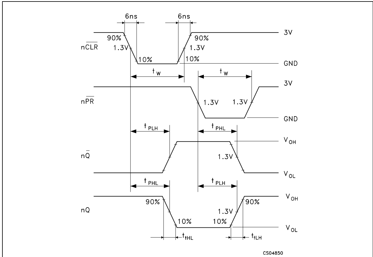
WAVEFORM 2 : MINIMUM PULSE WIDTH, PROPAGATION DELAY ( f=1\text{MHz} ; 50% duty cycle)
