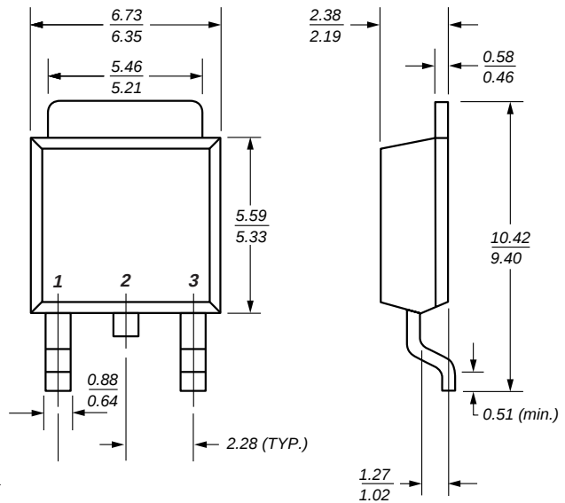
TO-252 (DPAK)
