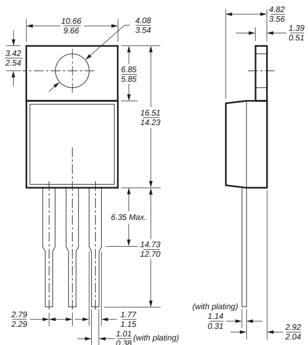
TO-220
