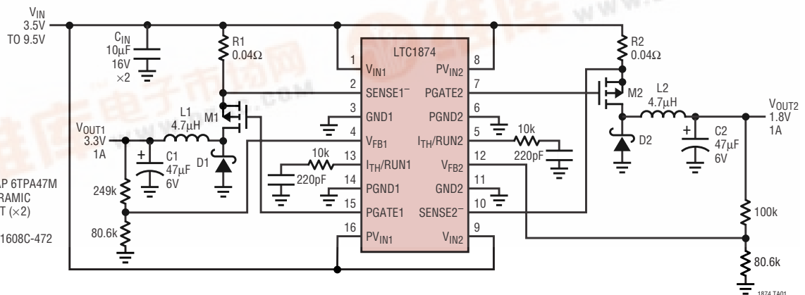
Figure 1. LTC1874 3.5V-9.5V Input to 3.3V/1A and 1.8V/1A Dual Step-Down Converter
