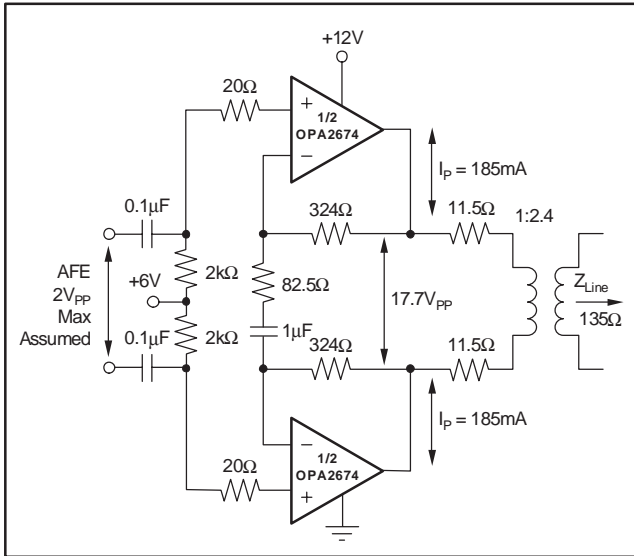
Figure 6. HDSSL2 Upstream Driver
