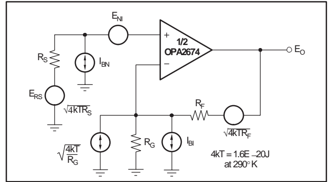
Figure 13. Op Amp Noise Analysis Model
