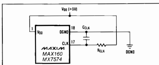
Figure 8. Connecting R_{CLK} and CLK to CLK Oscillator
