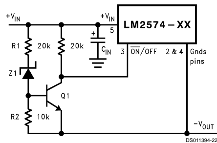
FIGURE 14. Undervoltage Lockout for Buck-Boost Circuit
