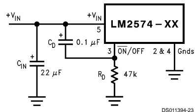
FIGURE 15. Delayed Startup
