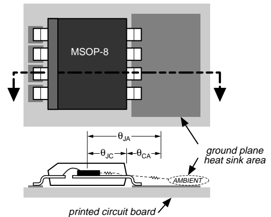
Figure 3. Thermal Resistance
