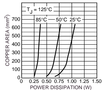
Figure 5. Copper Area vs. Power-MSOP Power Dissipation ( T_A )
