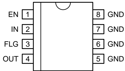
MIC3775-x.x Fixed MSOP-8 (MM)
