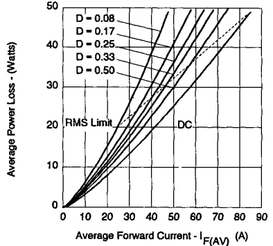
Fig. 6 - Forward Power Loss Characteristics
