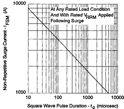
Fig. 7 - Maximum Non-Repitative Surge Current
