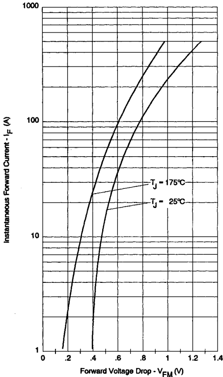
Fig. 1 - Maximum Forward Voltage Drop Characteristics
