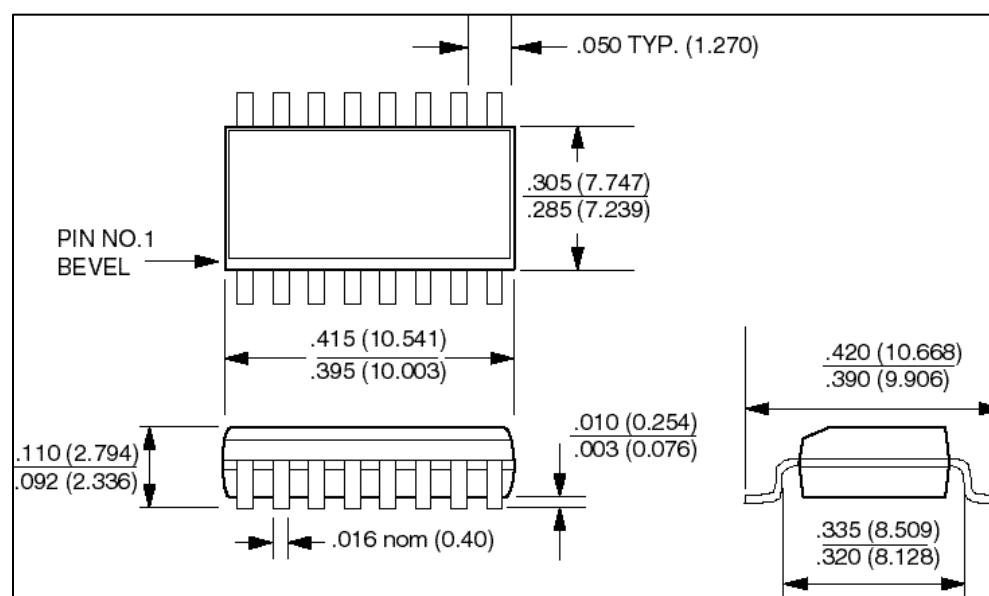
16-Pin SOL
