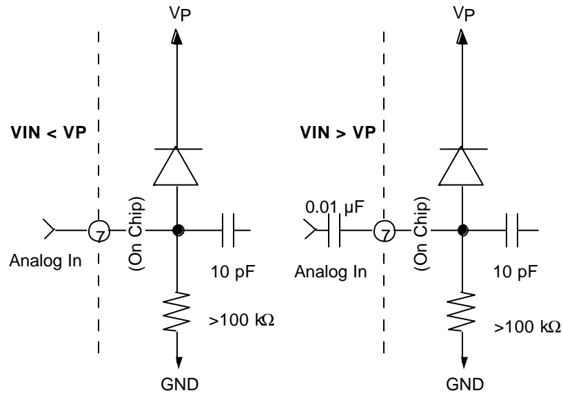
FIGURE 1: Input Coupling
