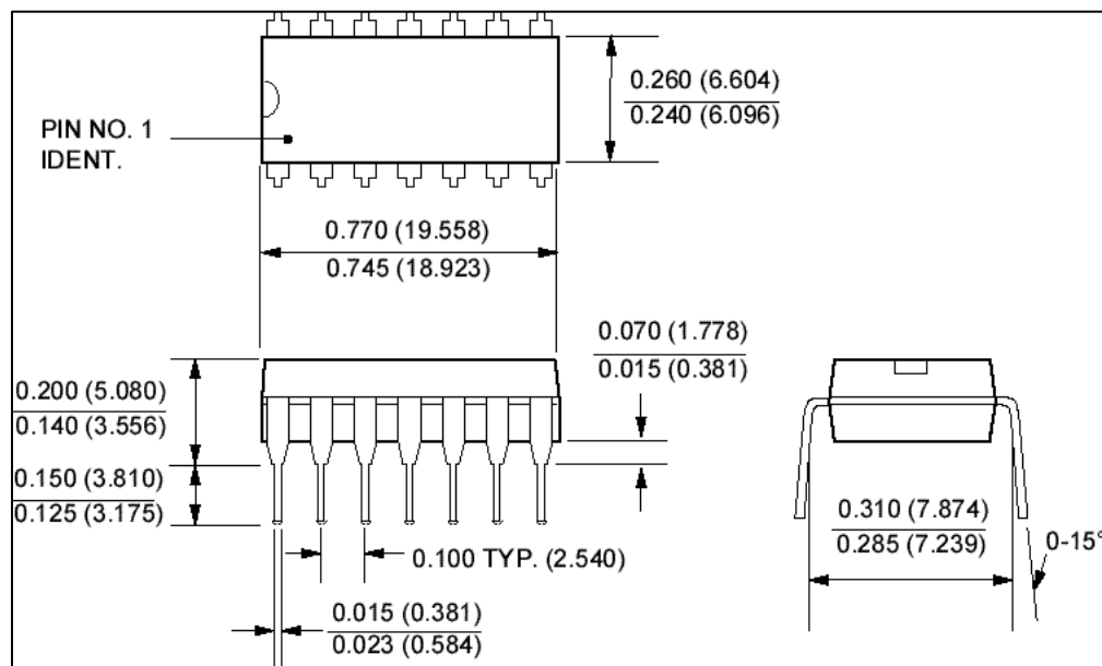
14-Pin DIP
