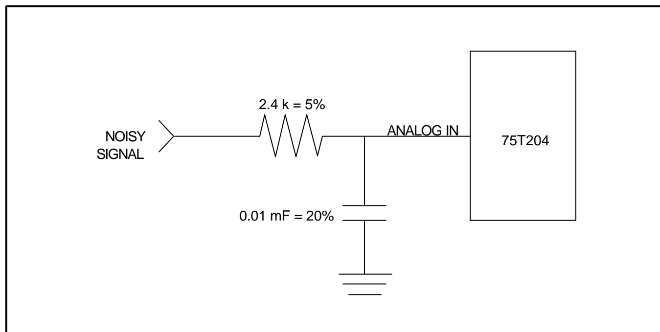
FIGURE 5: RC Filter
