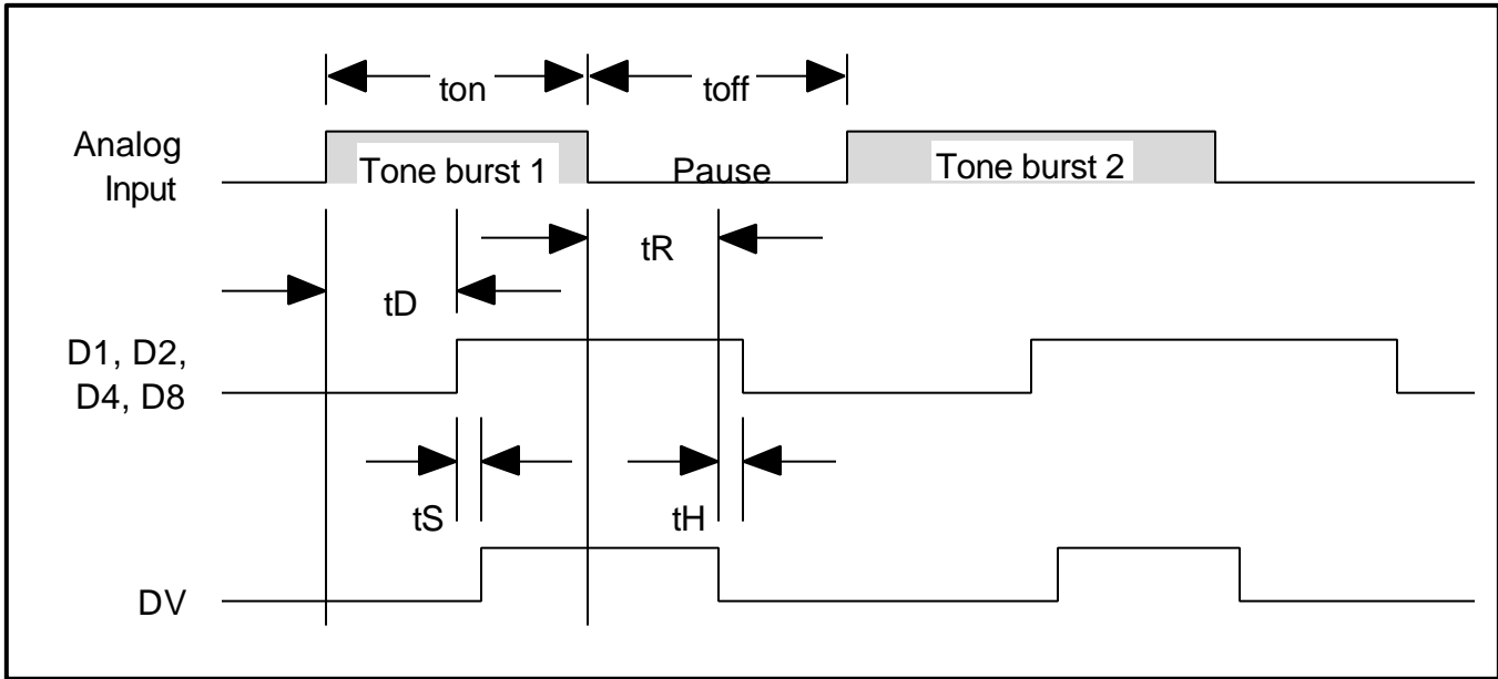
FIGURE 4: Timing Diagram
