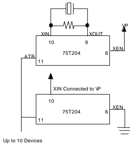
FIGURE 2: Crystal Connections
