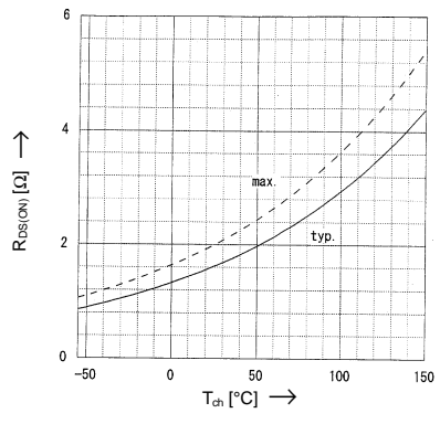
Drain-Source-On-State Resistance vs. T_{ch} R_{DS(on)} = f(T_{ch}) ; I_D = 3.5\text{A} ; V_{GS} = 10\text{V}
