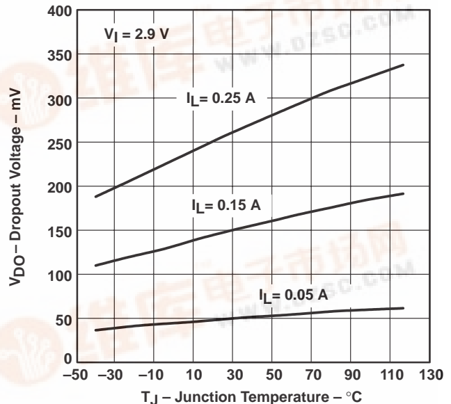
TPS77930 DROPOUT VOLTAGE vs JUNCTION TEMPERATURE
