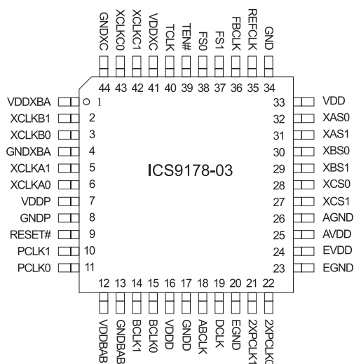
44-Pin PQFP
