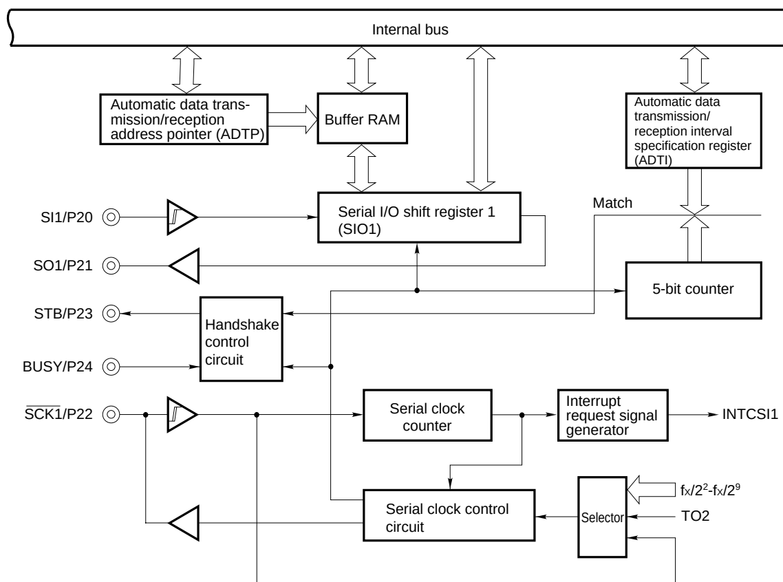
Fig. 5-11 Serial Interface Channel 1 Block Diagram
