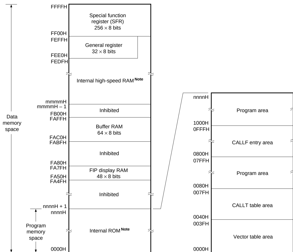
Fig. 4-1 Memory Map
