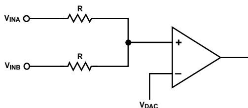
Figure 3. AD7883 Input Circuit
