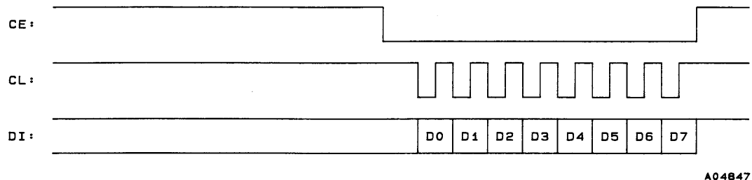
Serial input format 2 (CCB = low)
