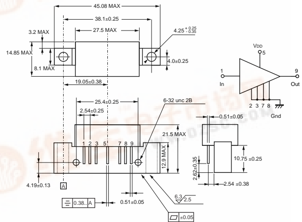
PACKAGE OUTLINE H02
