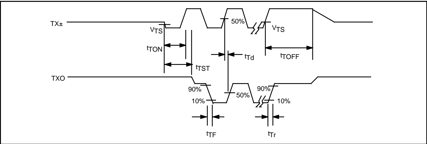
FIGURE 4: Transmitter Timing
