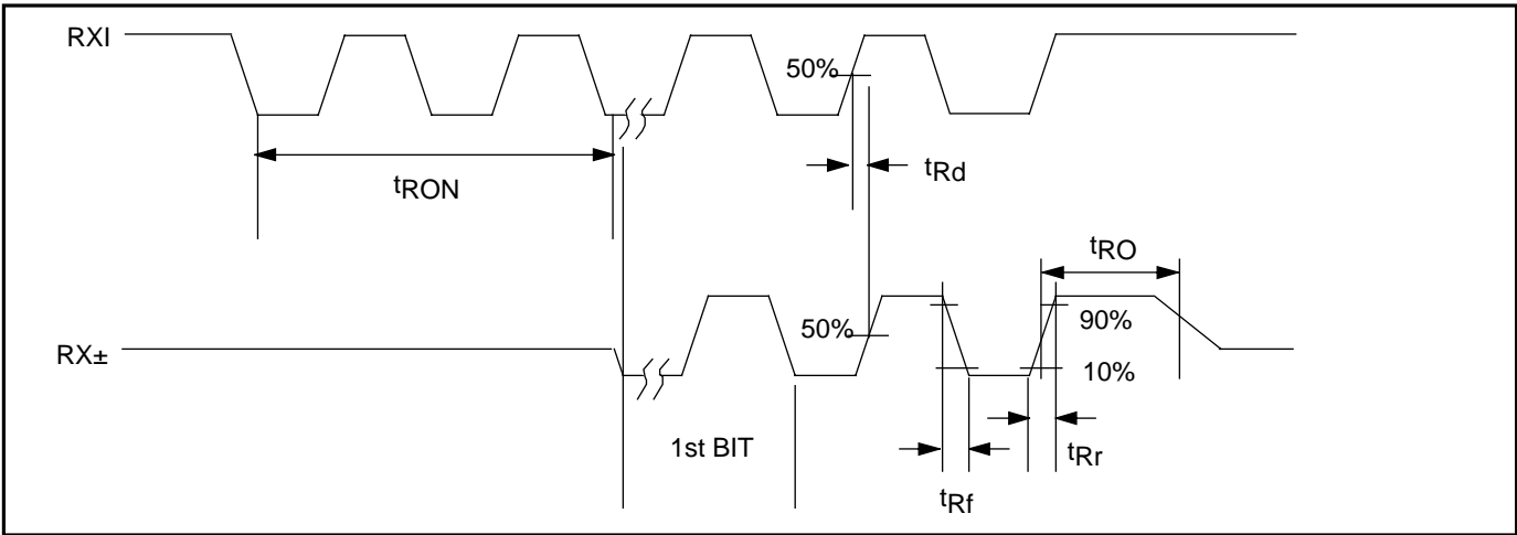
FIGURE 3: Receiver Timing
