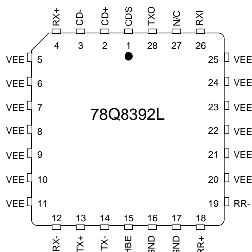
28-Pin PLCC
