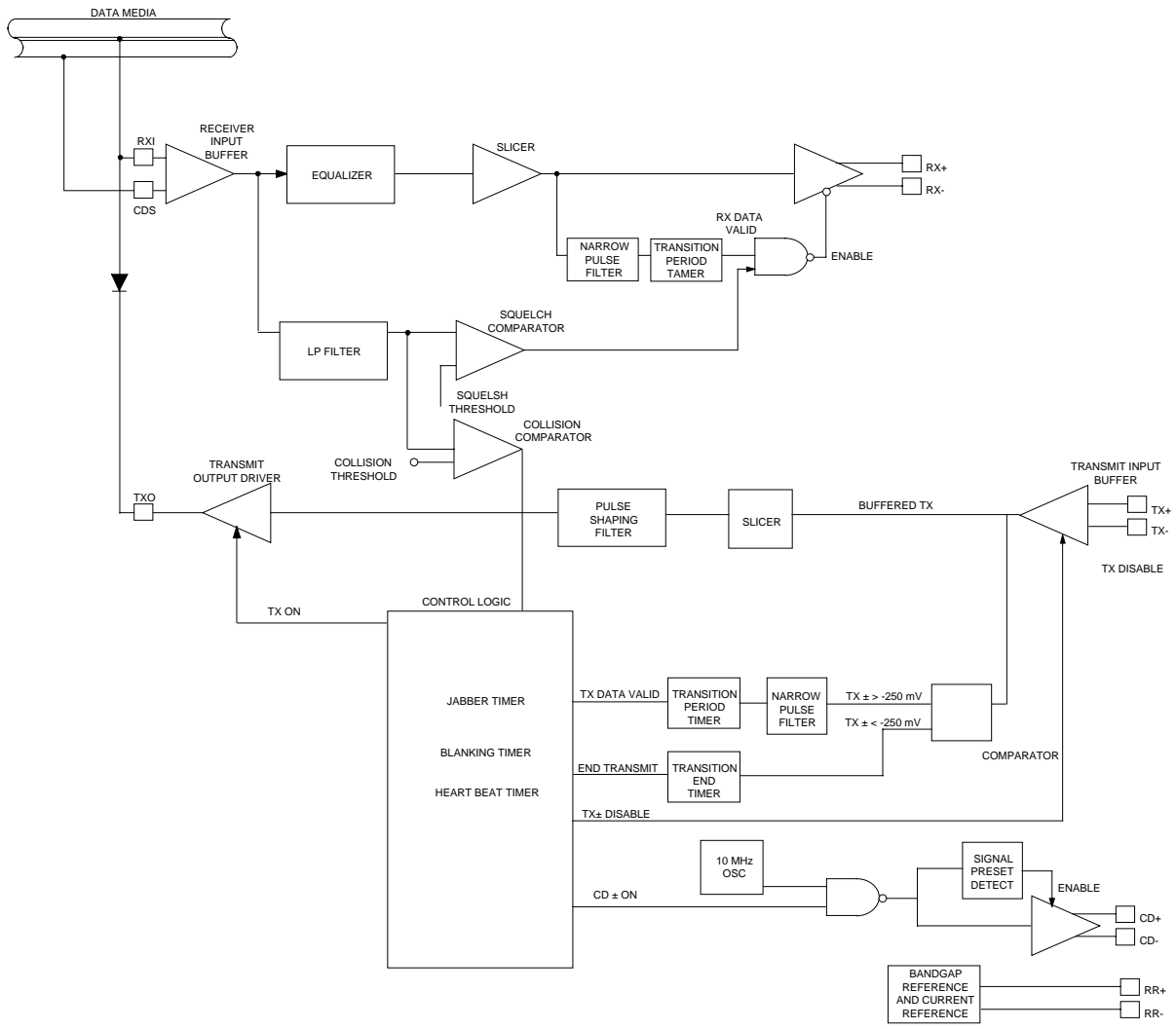
FIGURE 1: 78Q8392L General System Block Diagram
