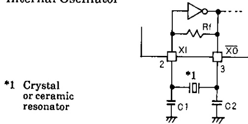
Fig. 1 Internal Oscillator
