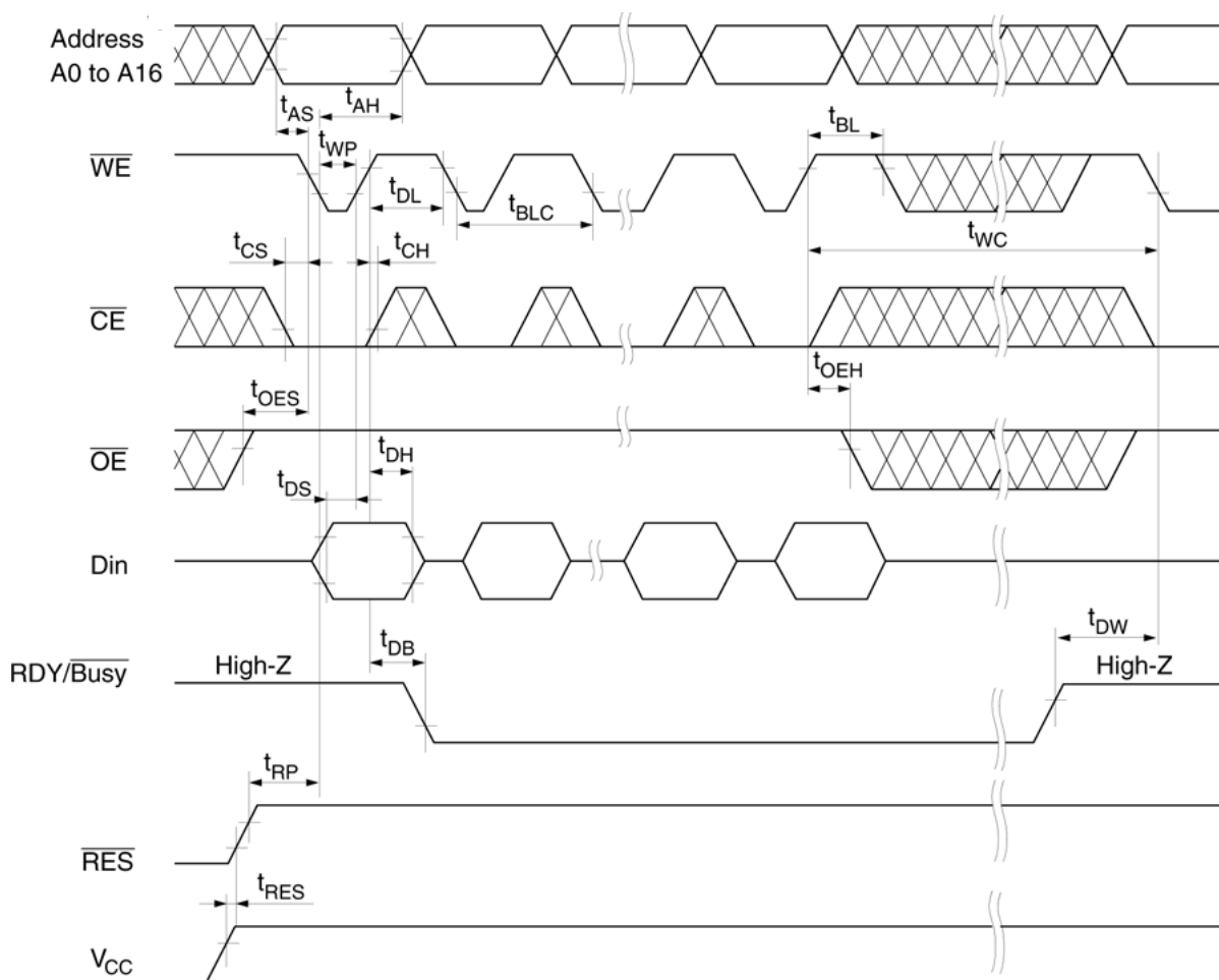
FIGURE 4. PAGE WRITE TIMING WAVEFORM(1) ( \overline{WE} CONTROLLED)
