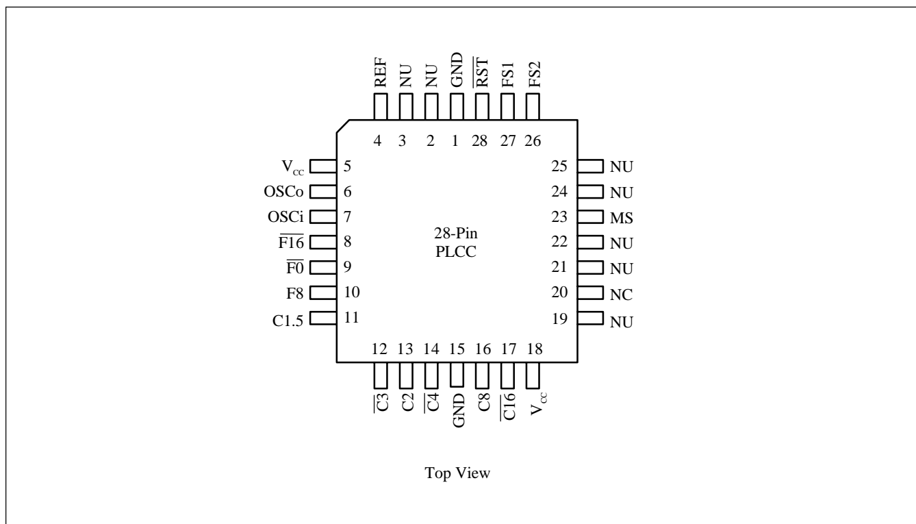
Figure 2. Pin Configuration
