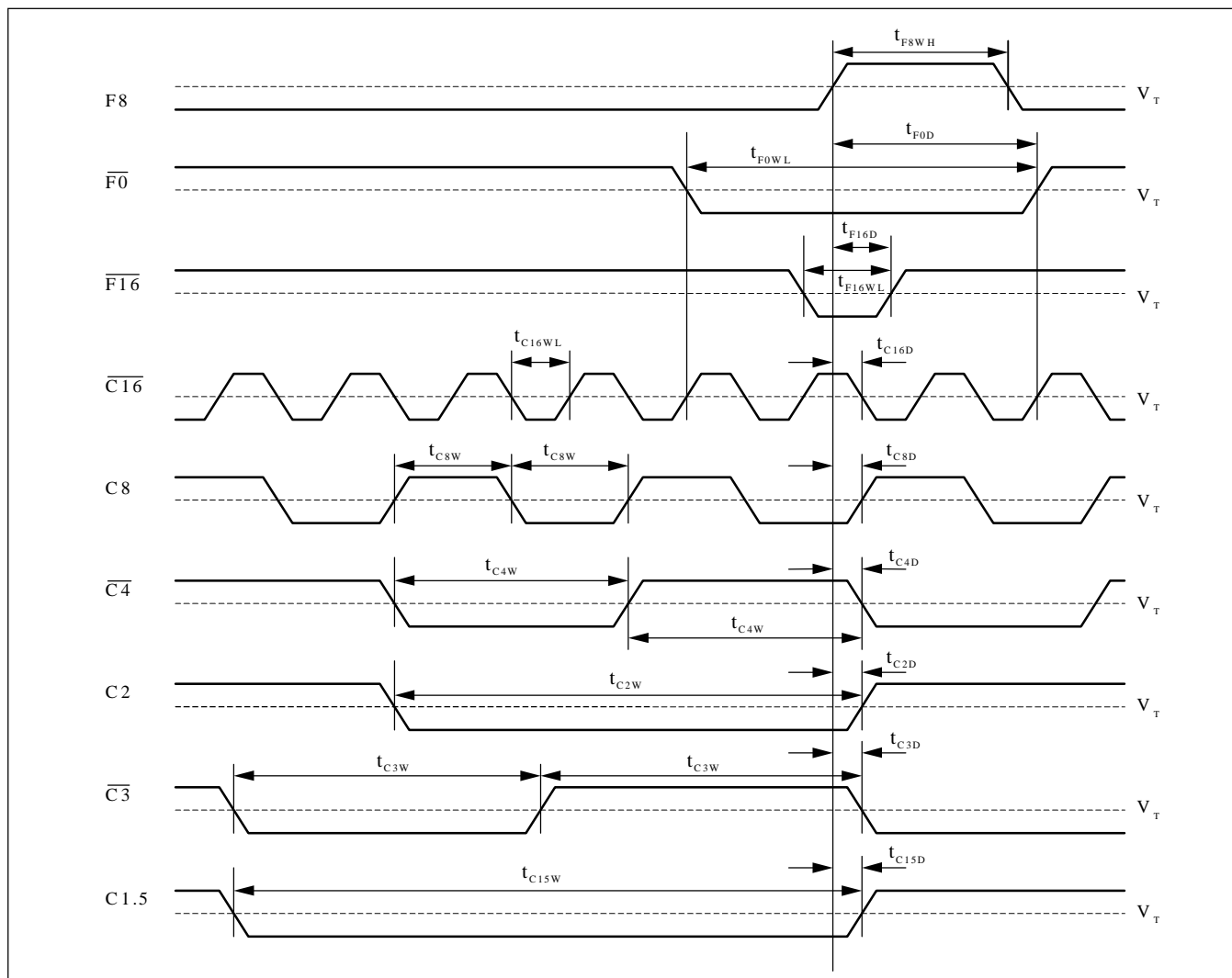
Figure 10. Output Timing
