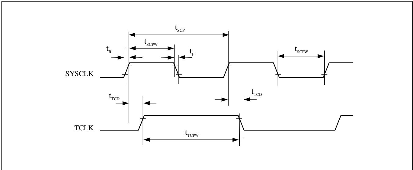
Figure 45. Clock Timing
