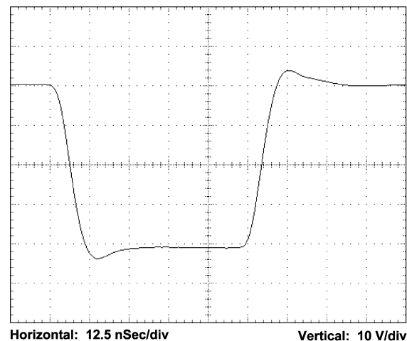
FIGURE 7. Red Cathode Response
