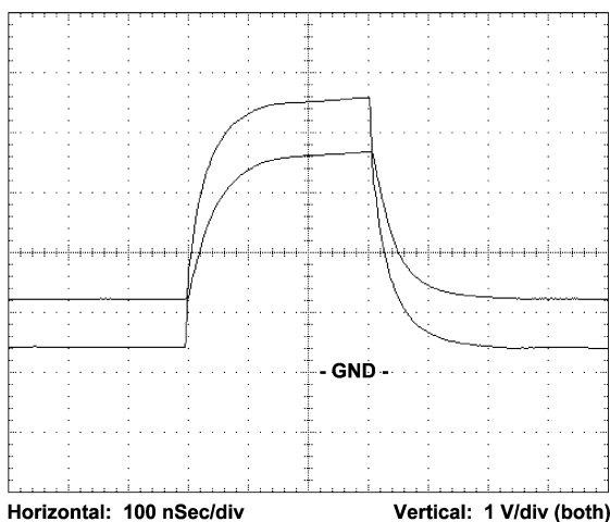
FIGURE 6. Logic Clamp Pulse
