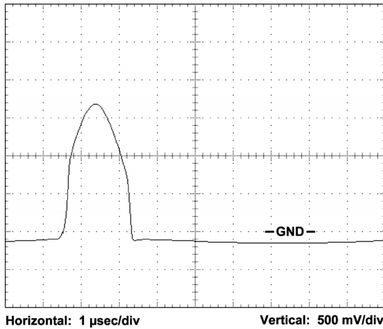
FIGURE 4. Deflection Horizontal Blanking
