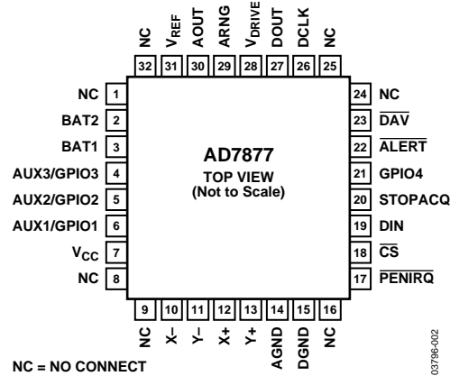
Figure 4. Pin Configuration
