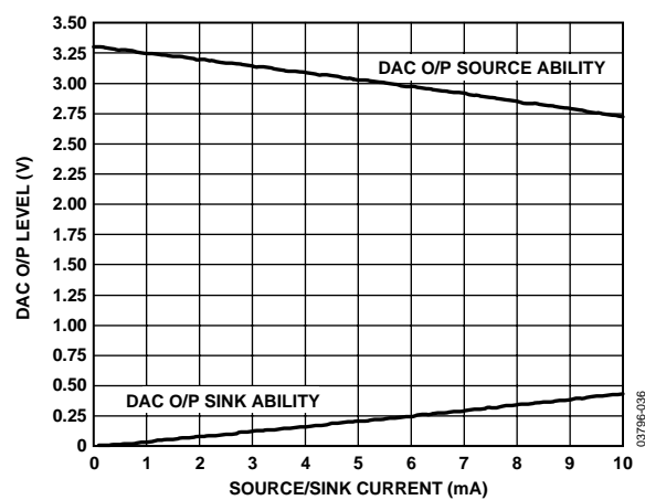
Figure 22. DAC Source and Sink Current Capability
