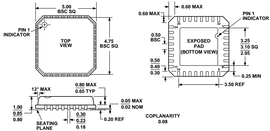
Figure 48. 32-Lead Lead Frame Chip Scale Package [LFCSP] 5 mm x 5 mm Body (CP-32-2) Dimensions shown in millimeters
