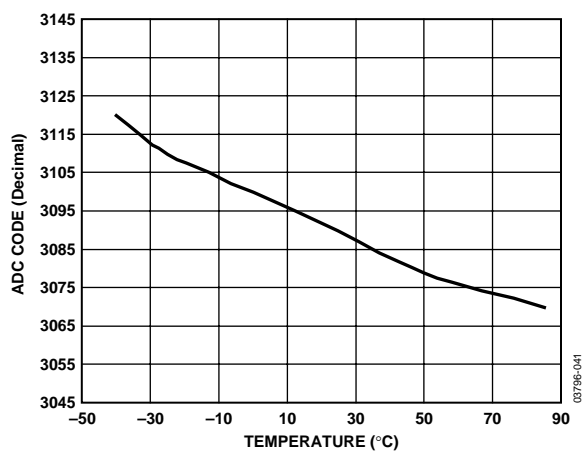
Figure 17. ADC Code vs. Temperature (2.7 V Supply)
