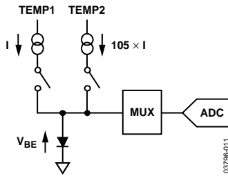
Figure 32. Block Diagram of Temperature Measurement Circuit
