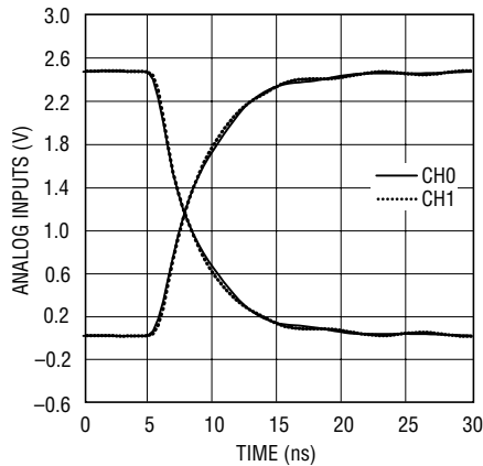
Simultaneous Input Steps at CH0 and CH1 from 25\Omega
