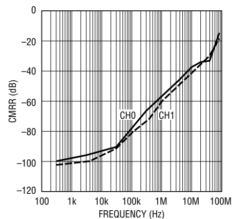
Figure 3. CMRR vs Frequency
