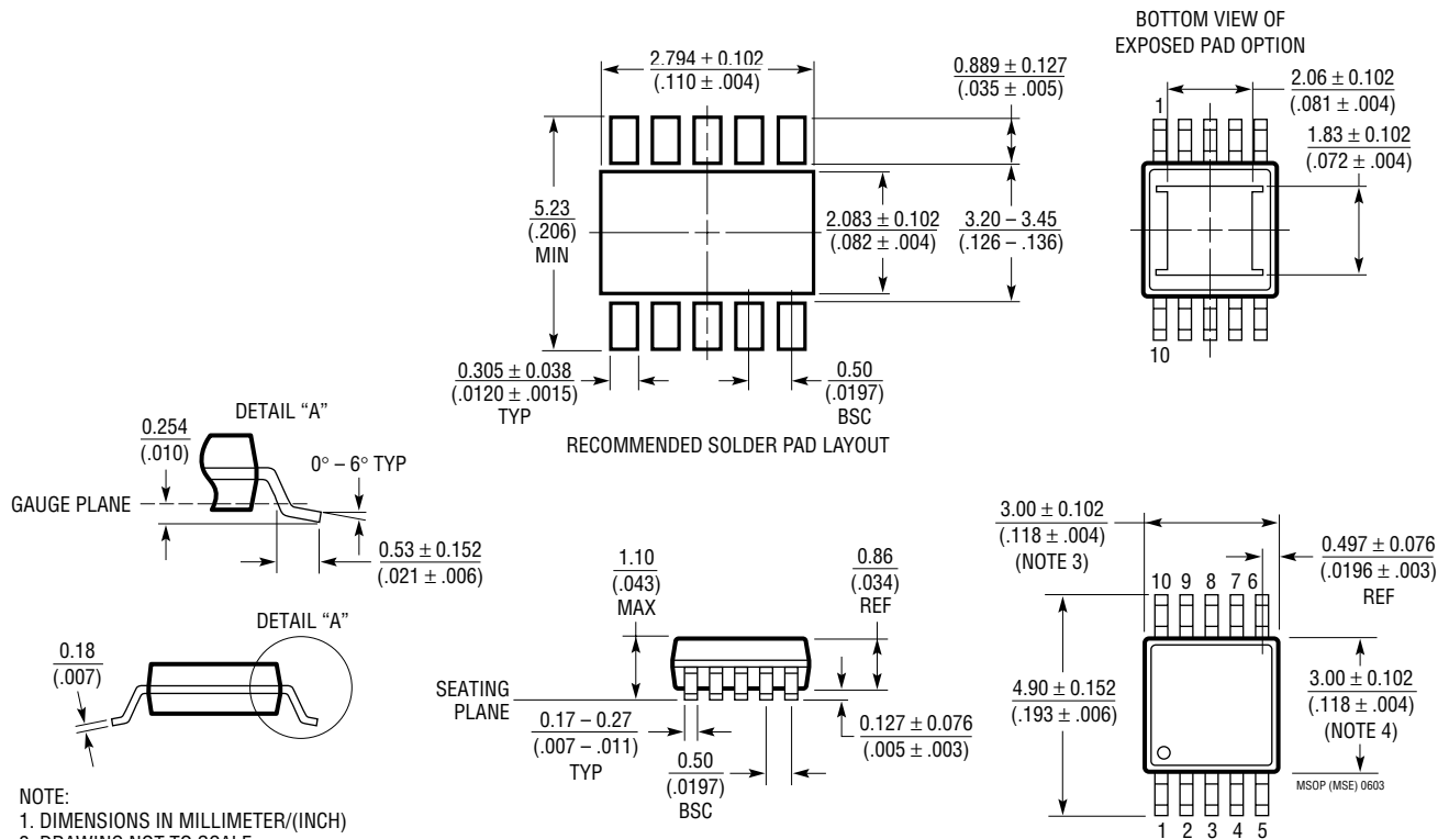
MSE Package 10-Lead Plastic MSOP (Reference LTC DWG # 05-08-1663)
