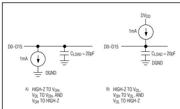
Figure 1. Load Circuits
