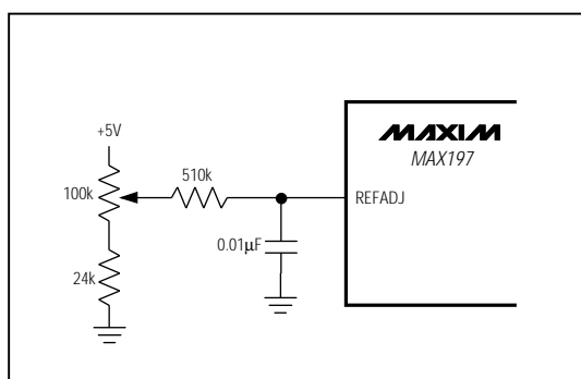
Figure 1. Reference-Adjust Circuit
