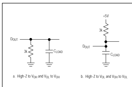
Figure 2. Load Circuits for Enable Time
