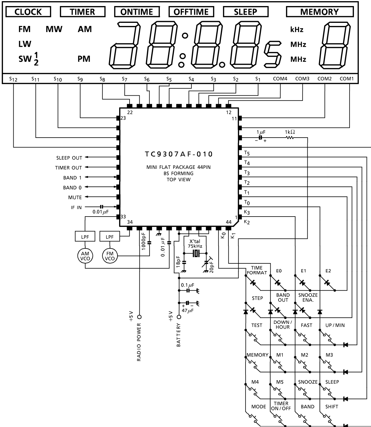
TC9307AF-010 Layout
