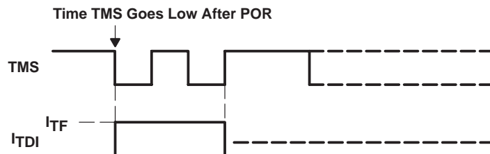
Figure 7. Fuse Check Mode Current, MSP430P337A
