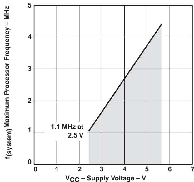
Figure 2. Processor Frequency vs Supply Voltage
