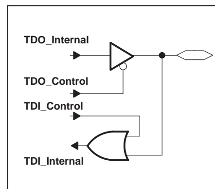
MSP430C33x: TDO/TDI MSP430P/E337A: TDO/TDI
