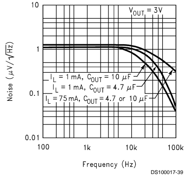
Output Noise Density (LP2987)
