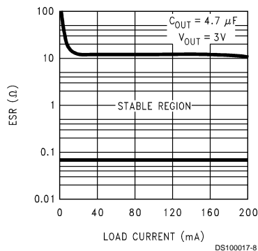
ESR Curves For 3V Output
