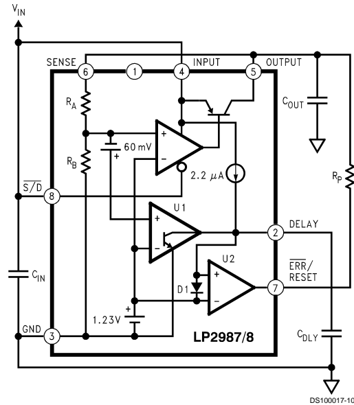
LP2987/8 Equivalent Circuit
