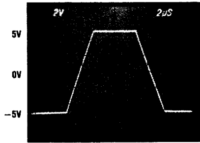
OP-27 Large Signal Transient Response
