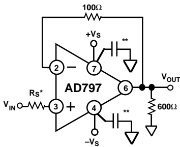
Figure 22. Follower Connection
