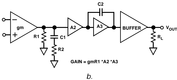
Figure 27. Model of AD797 vs. That of a Typical Three-Stage Amplifier
