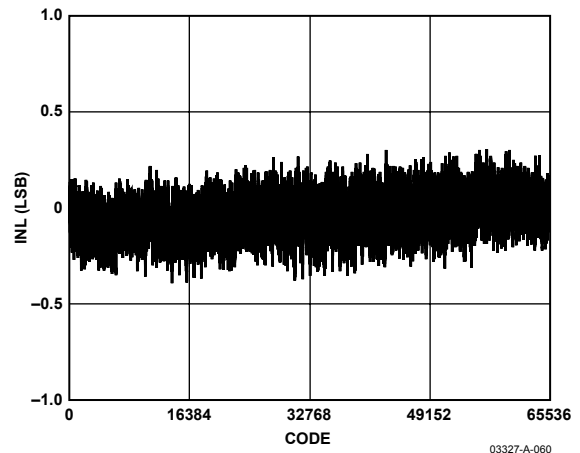
Figure 61. Integral Nonlinearity
