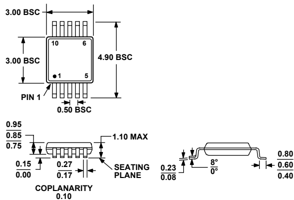
Figure 66. 10-Lead Mini Small Outline Package [MSOP] (RM-10) Dimensions shown in millimeters
