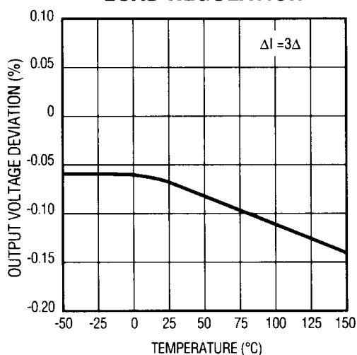
LOAD REGULATION
