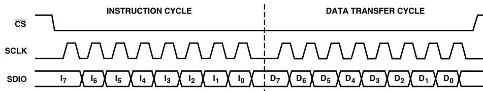
Figure 27. Serial Port Writing Timing—Clock Stall Low
