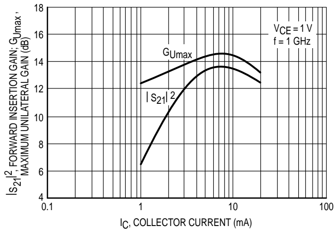
Figure 10. Maximum Unilateral Gain and Forward Insertion Gain versus Collector Current
