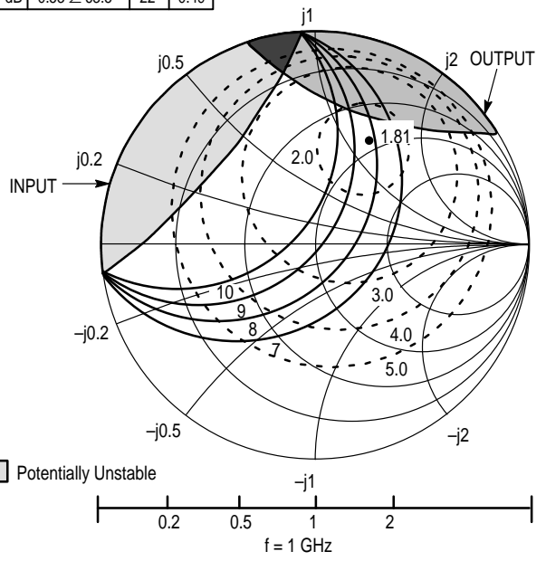
Figure 23. MRF2947 Series Constant Gain and Noise Figure Contours
