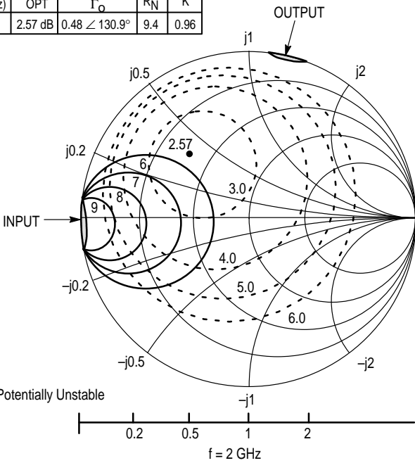
Figure 22. MRF2947 Series Constant Gain and Noise Figure Contours
