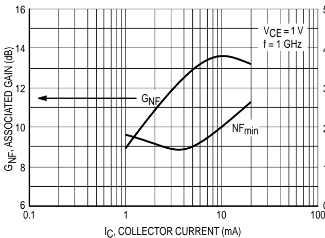
Figure 16. Minimum Noise Figure and Associated Gain versus Collector Current
